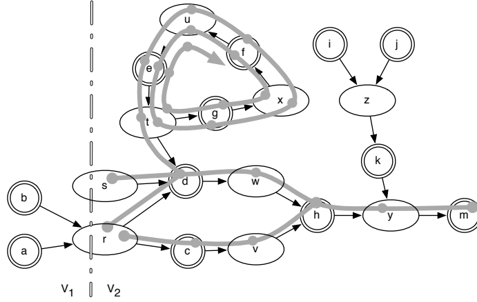
Figure 12: A cut-limited inverted tree rooted at vertex m .
