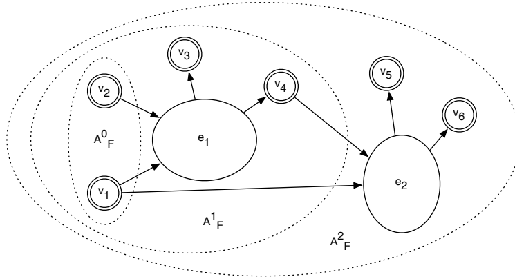
Figure 9: A_F^k for A = \{v_1, v_2\} and F = \{e_1, e_2\} .
