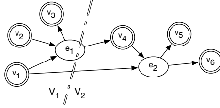
Figure 11: Cross(c) = \{e_1\} , where c = (\{v_1, v_2, v_3\}, \{v_4, v_5, v_6\})
