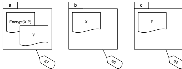
Figure 6: Formula a \triangleright_4 b \rightarrow (\emptyset \triangleright_4 b \vee b \triangleright_4 a) is false.
