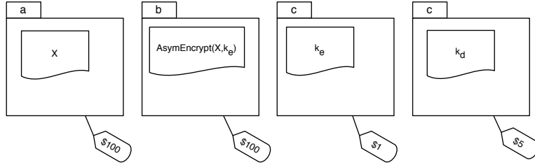
Figure 7: Formula a \triangleright_1 b \wedge b \triangleright_5 a \rightarrow (\emptyset \triangleright_5 a \vee \emptyset \triangleright_1 b \vee b \triangleright_4 a) is false.
