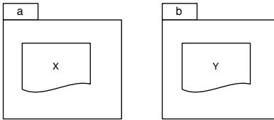
Figure 2: Formulas a \triangleright b and b \triangleright a are both false.
