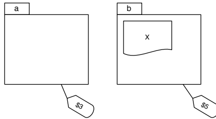
Figure 4: Formula a \triangleright_4 b is false.
