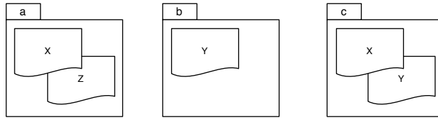
Figure 3: Formula a, b \triangleright c is true.
