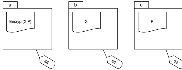
Figure 5: Formula a \triangleright_4 b \rightarrow \emptyset \triangleright_4 b is false.
