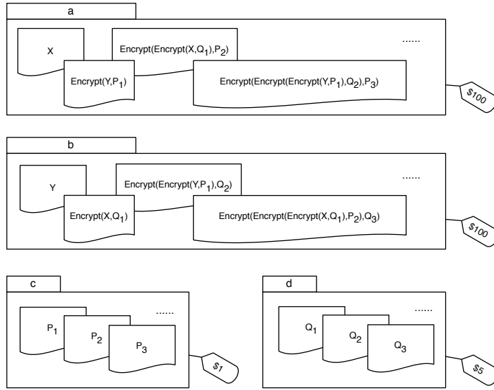
Figure 8: Formula a \triangleright_1 b \wedge b \triangleright_5 a \rightarrow (\emptyset \triangleright_5 a \vee \emptyset \triangleright_1 b \vee b \triangleright_4 a) is false.
