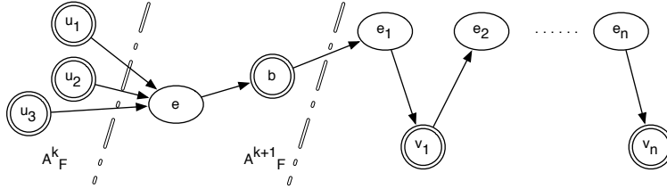
Figure 10: Illustration to Lemma 10.
