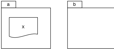
Figure 1: Formula a \triangleright b is true, but formula b \triangleright a is false.
