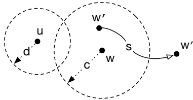
Figure 7: Illustration of Lemma 19.
